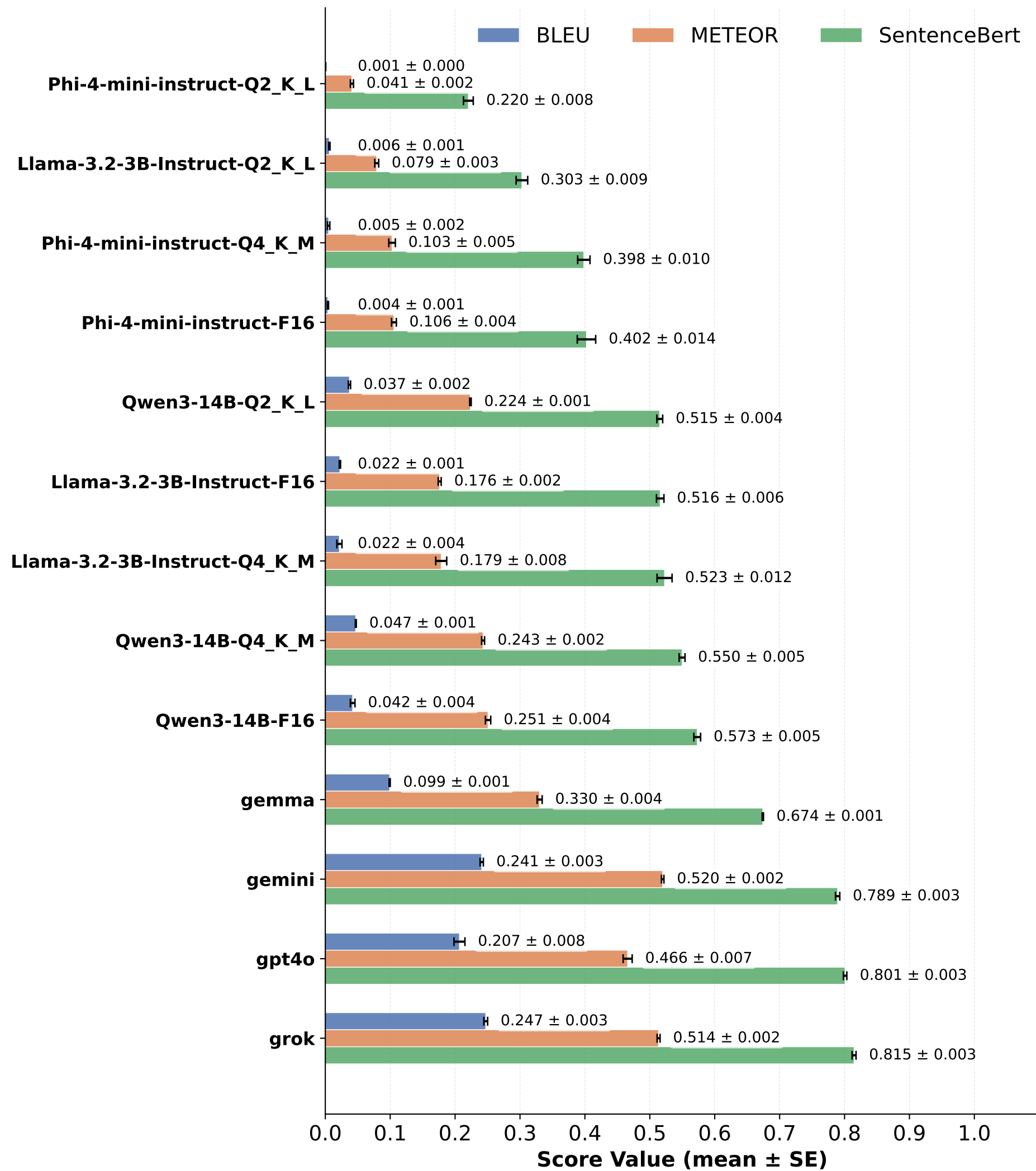
Average Translation Metrics by Model
